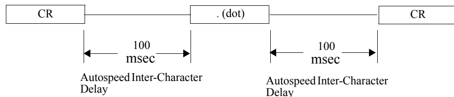
Figure 6. Autospeed Inter-Character Delay
