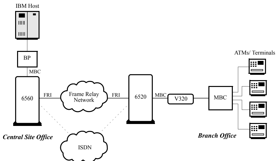
Figure 3. MBC Protocol Support on 6560
