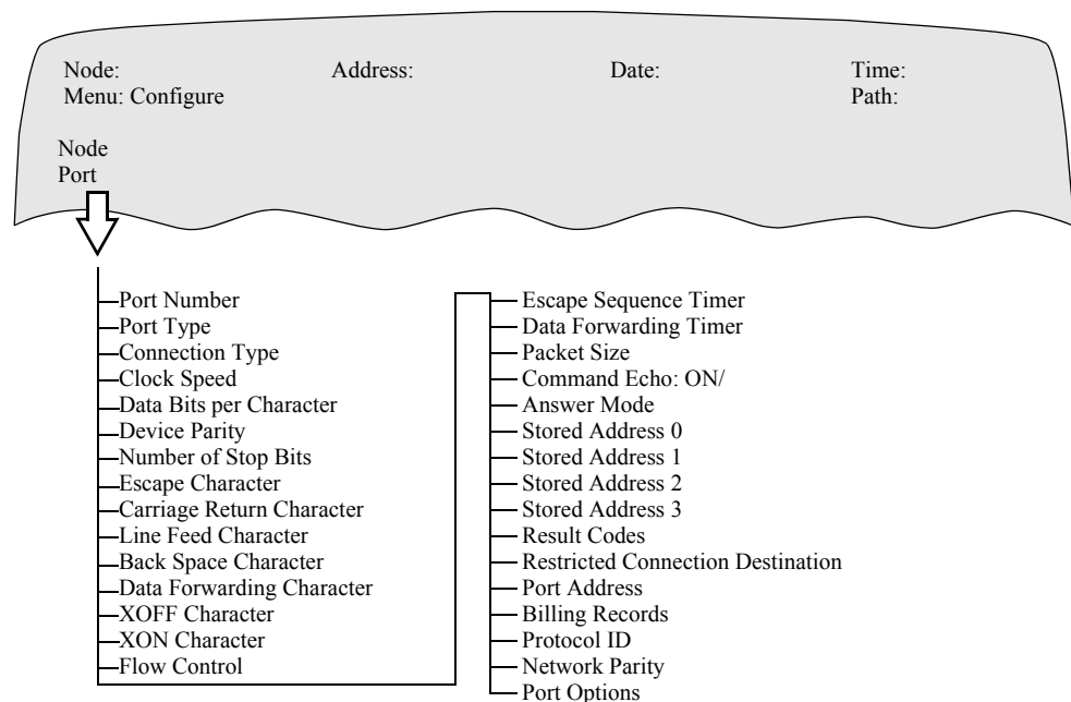
Figure 15. Configure ATPAD Port Menu
