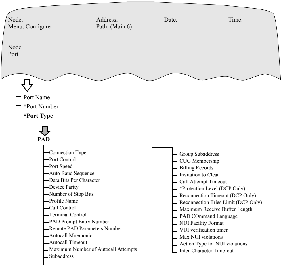
Figure 4. PAD Port Record
